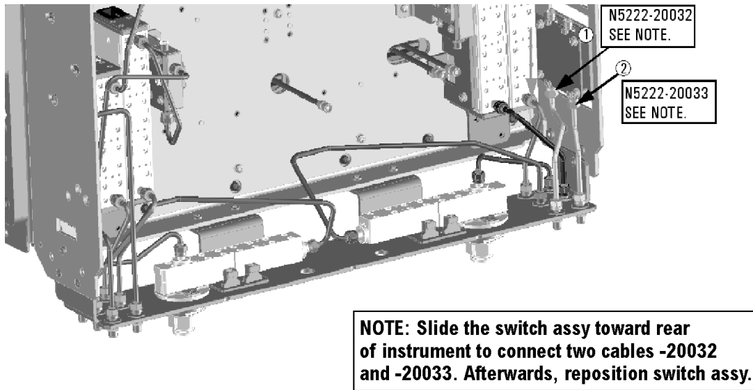
Figure 3 Instructions to Install W36
